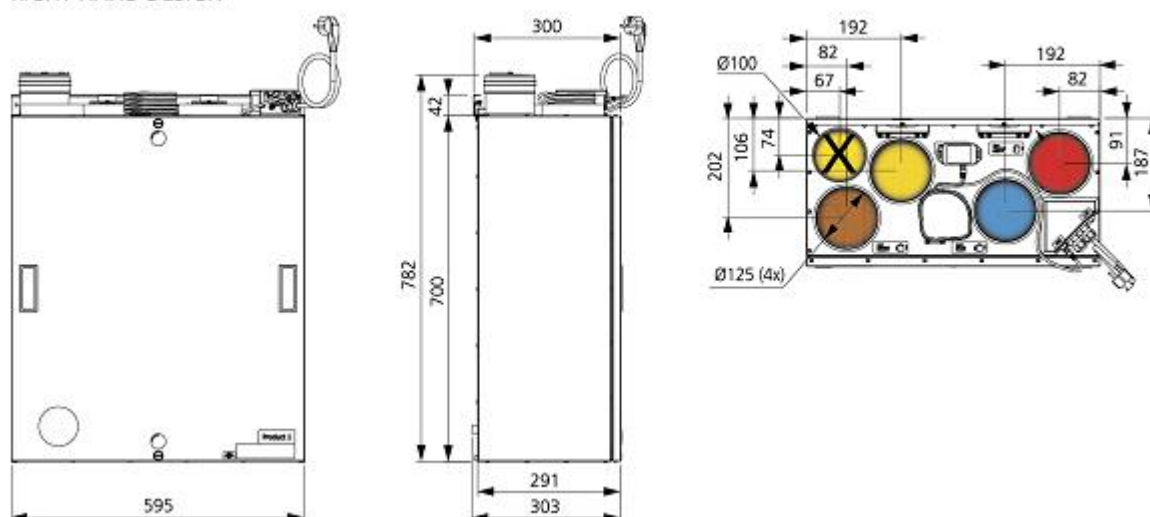
RIGHT-HAND DESIGN
